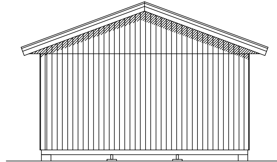
FASAD GAVEL 1
